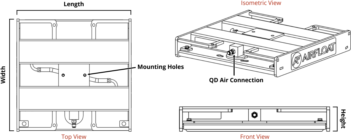
Isometric View
