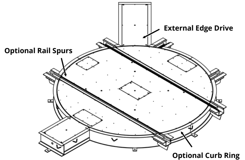
Isometric View
